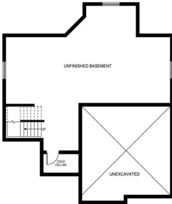
FOUNDATION PLAN
