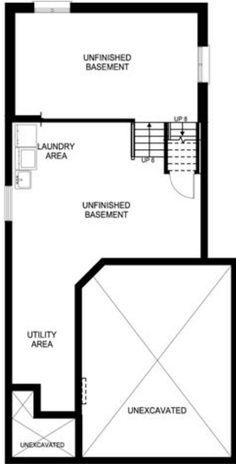
FOUNDATION PLAN
