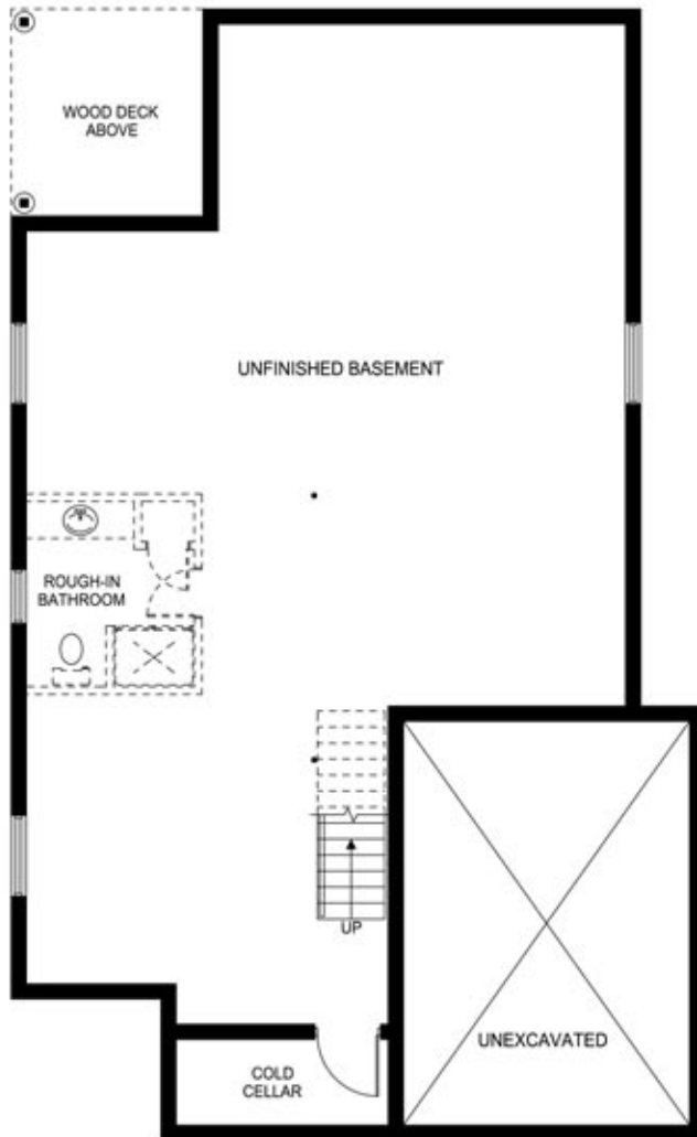
FOUNDATION PLAN
